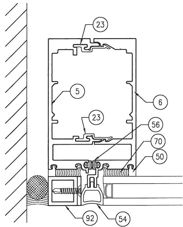
11 ALTERNATE JAMB GLAZING BUTT GLAZED Scale: 6" = 1'-0"
