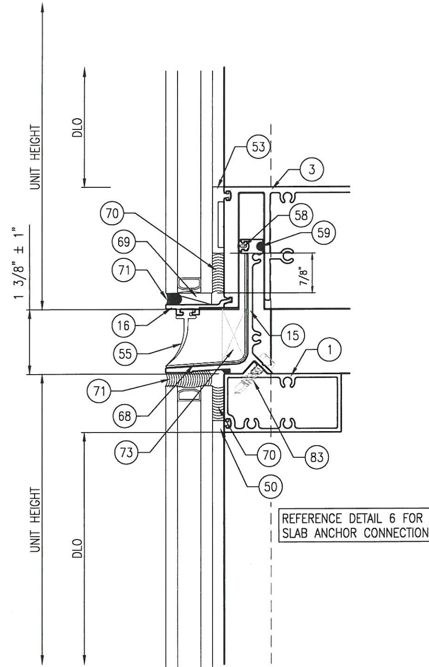
7 STACK JOINT (BUTT-GLAZED) SECTION Scale: 6" = 1'-0"
