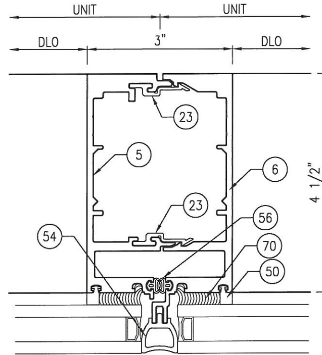
4A MULLION (BUTT-GLAZED) Scale: 6" = 1'-0"
