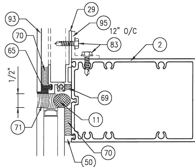
18A PANEL AT HORIZONTAL BUTT GLAZED Scale: 6" = 1'-0"
