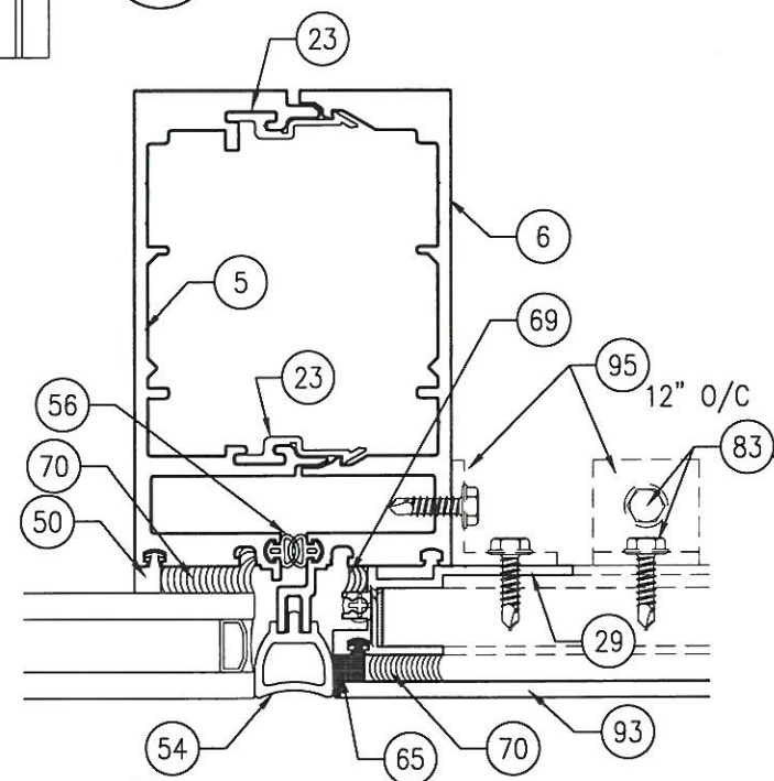
13 PANEL AT VERTICAL BUTT GLAZED Scale: 6" = 1'-0"
