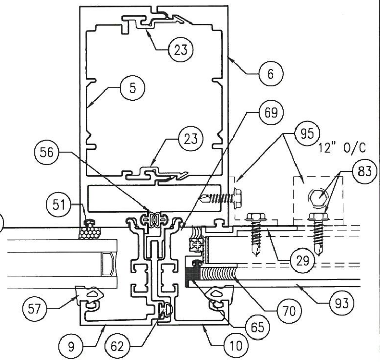
14 PANEL AT VERTICAL CAPTURED Scale: 6" = 1'-0"
