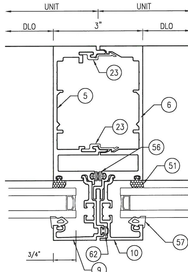
4 MULLION (CAPTURED) Scale: 6" = 1'-0"
