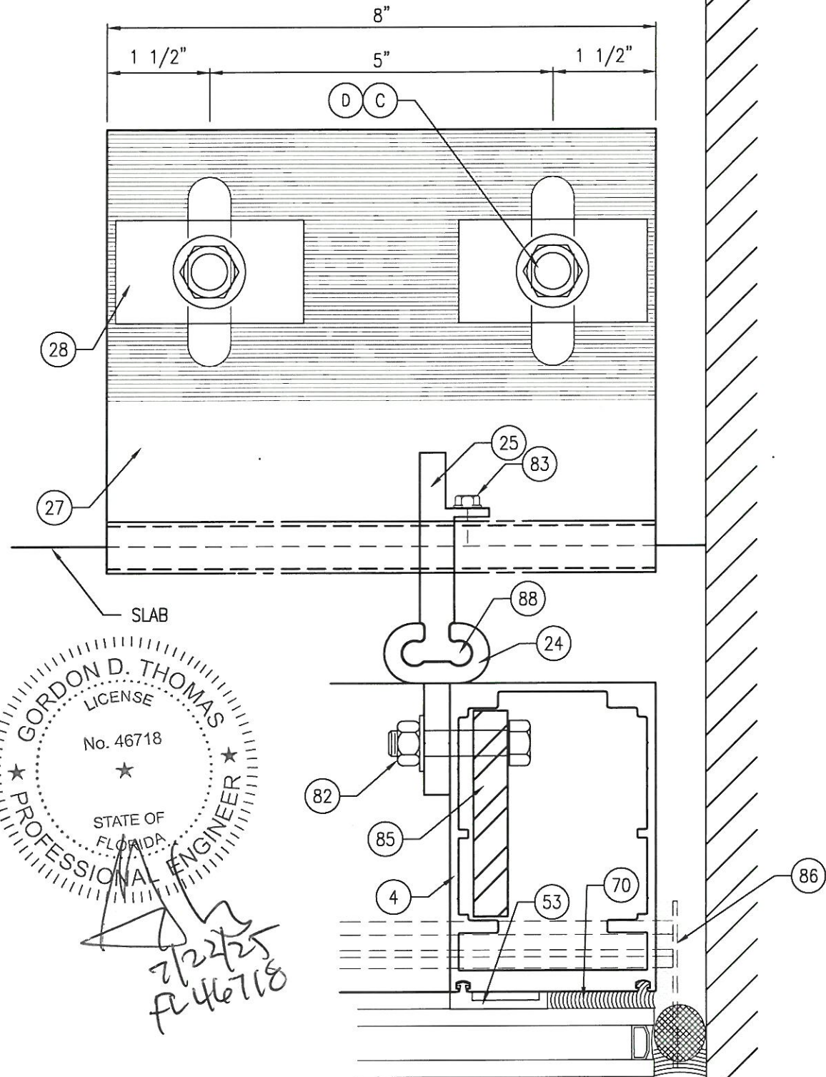
9A ANCHOR AT JAMB (BUTT-GLAZED) CONCRETE AND STEEL Scale: 6" = 1'-0"
