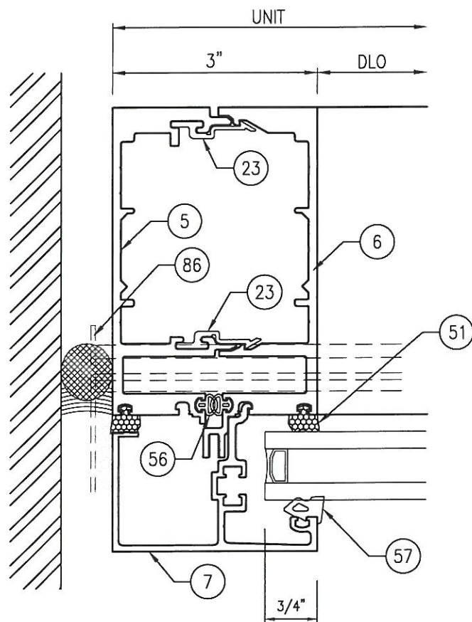
3 JAMB (CAPTURED) Scale: 6" = 1'-0"
