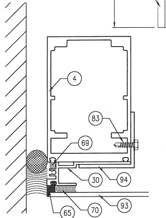
12 PANEL AT JAMB BUTT GLAZED Scale: 6" = 1'-0"
