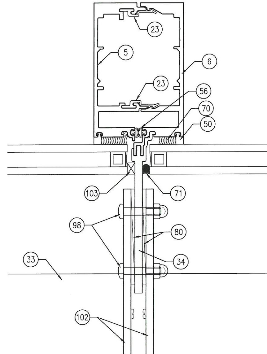
21 SUNSHADE CLIP TYPICAL VERTICAL Scale: 1:1
